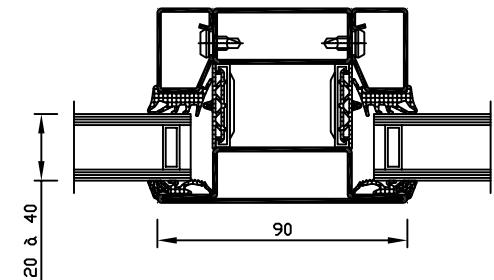
Montant - traverse Mullion - transom Pfosten - Riegel
